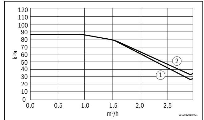
13. ábra CS2000AWF 4-6 R-S
