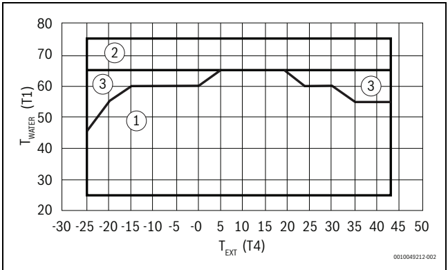
9. ábra CS2000AWF 4-6 R-S, CS2000AWF 8 -10 R-S, CS2000AWF 12-16 R-S/T
